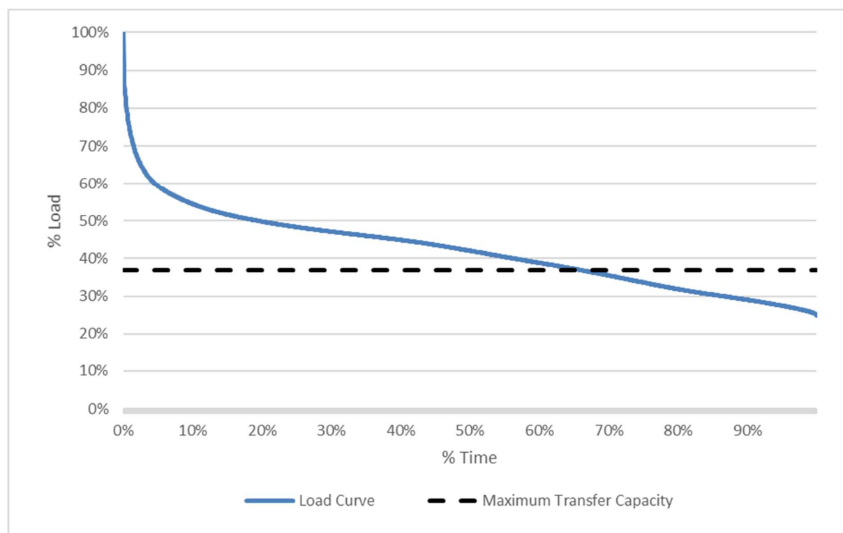
Figure C.1: Load duration curve for Concord Zone Substation
