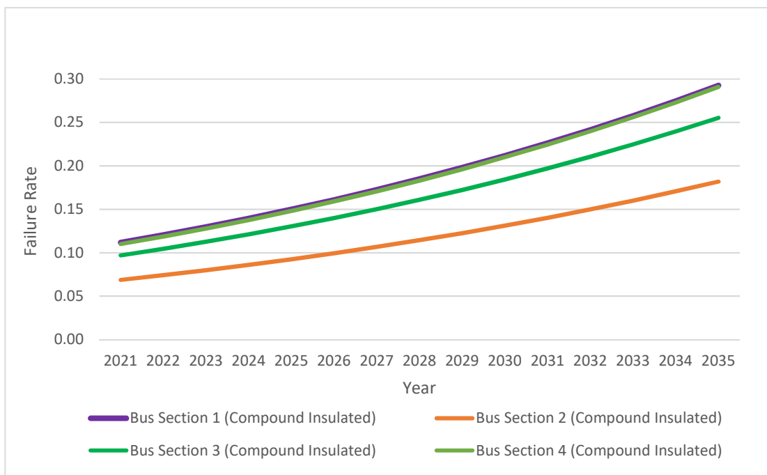
Figure C. 2: Cumulative probability of failure – 11kV switchboards
