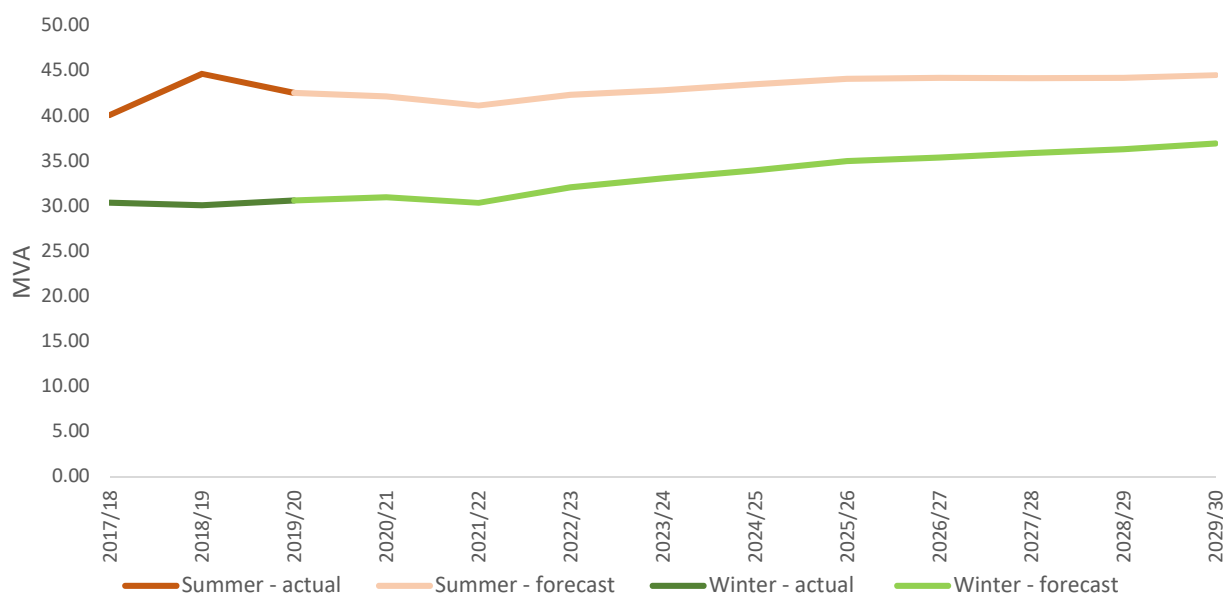
Figure 2-2 – Concord zone substation load
