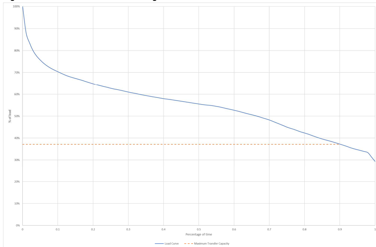
Figure D.1 – Load duration curve for Kingsford
