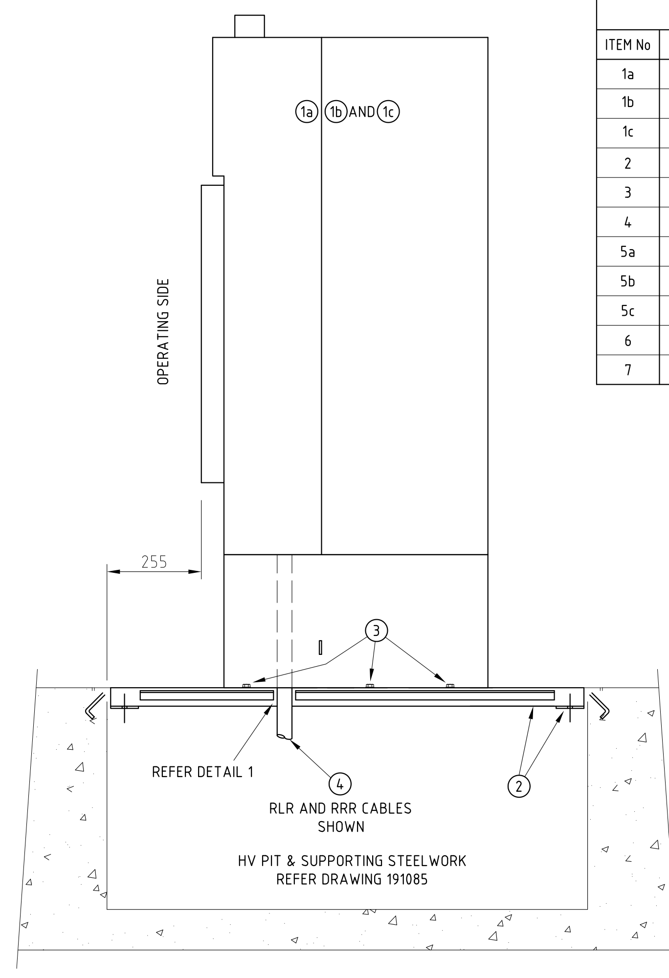
SECTION C-C ALL SWITCH VERSIONS SCALE 1:10
