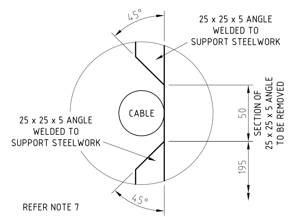
DETAIL 1 SUPPORTING STEELWORK MODIFICATION SCALE 1:2
