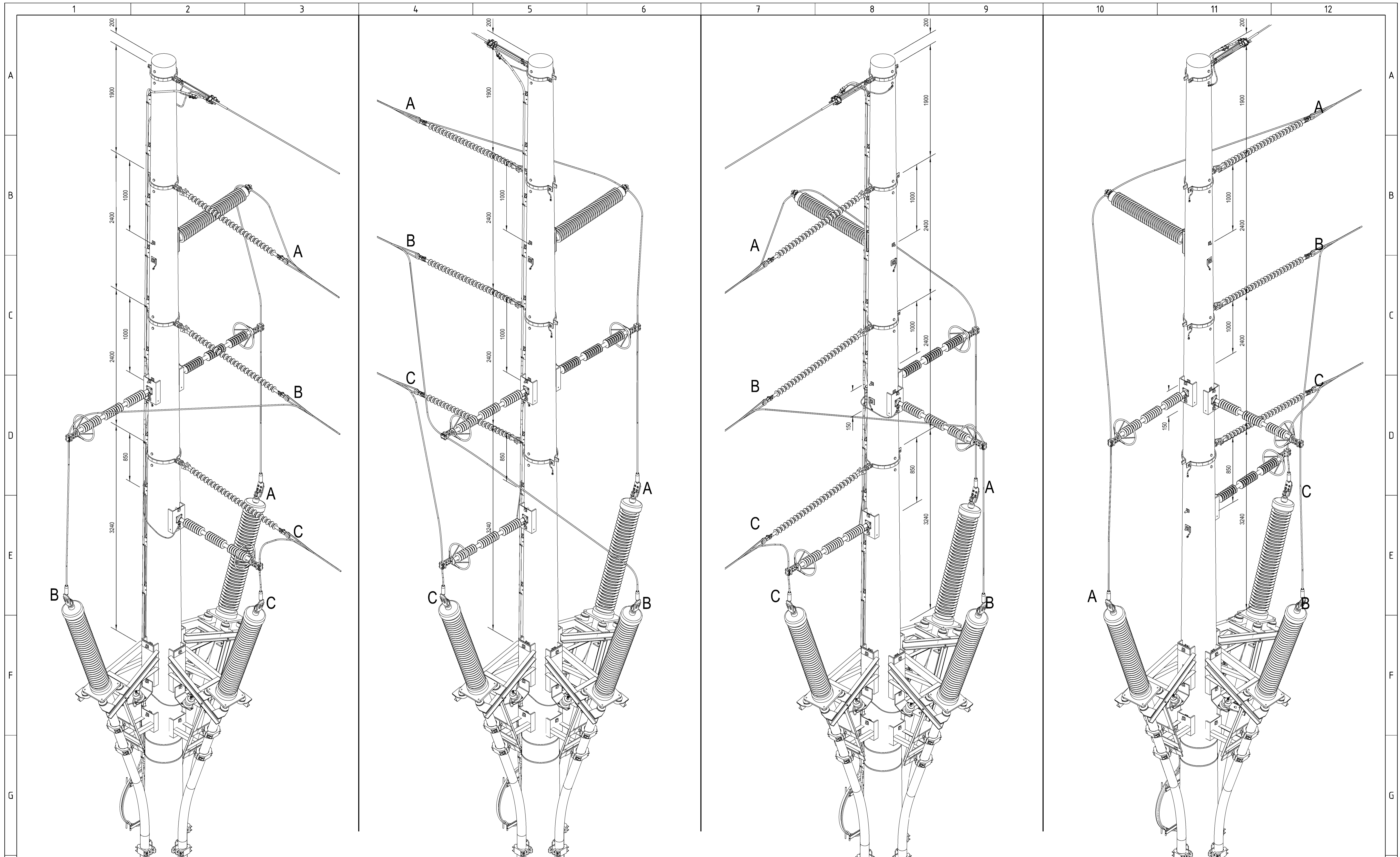
POLE TOP TYPE 1 (CABLE UP FRONT)
