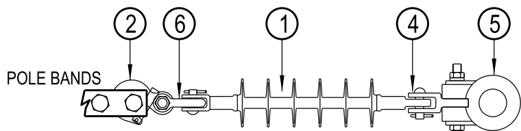
AR-4 - FLYING ANGLE
