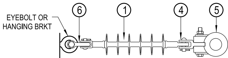
AR-1 - FLYING ANGLE OR SUSPENSION
