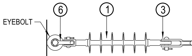
AR-2 - TERMINATION
